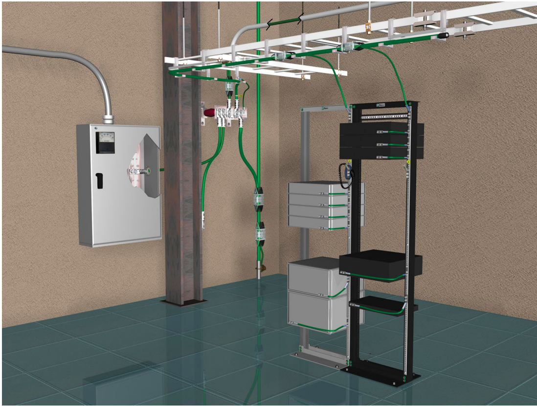
Figure 5: Grounding and Bonding in Telecommunications Room
